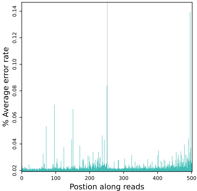
Error rate distribution along reads (R10620)
